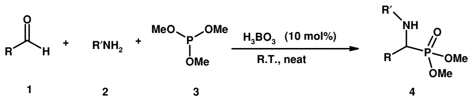
SCHEME 1 Synthesis of \alpha -aminophosphonates.
